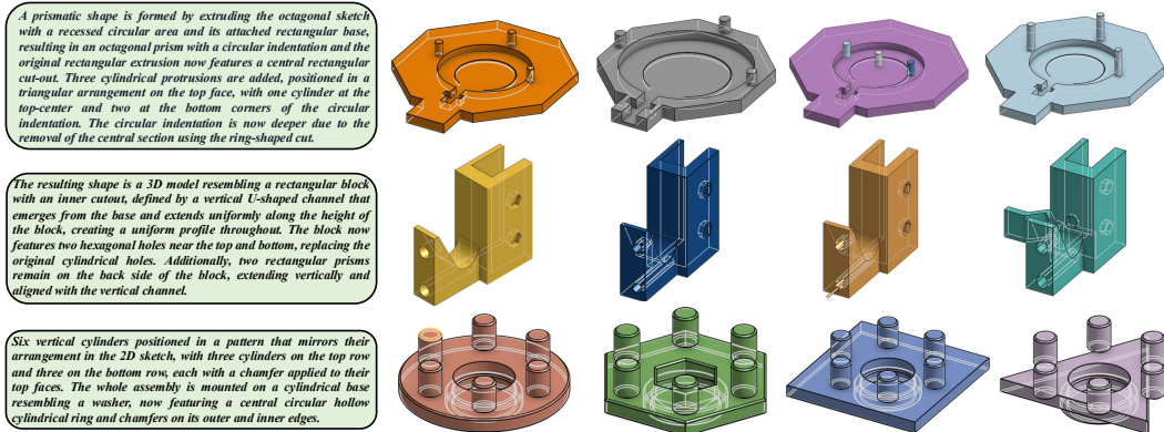
Figure 12: The showcases of similar generations.
