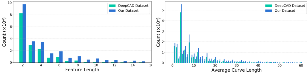
Figure 8: Statistical comparison between our complete dataset and the DeepCAD [54] dataset, which also is a subset of our dataset. The left plot illustrates the distribution of feature lengths, while the right plot shows the distribution of average curve lengths.
