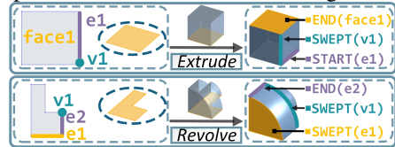
Figure 3: Illustration of the proposed CapType reference mechanism.
