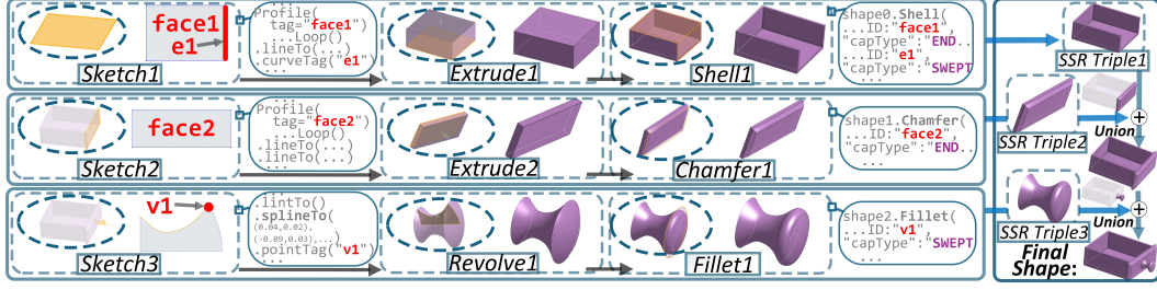
Figure 2: The SSR Design Paradigm. Each CAD model is constructed as a sequence of SSR triplets, where each triplet consists of a sketch , a sketch-based feature (e.g., extrude , revolve ), and optional refinement features (e.g., shell , chamfer , fillet ). Topological primitives are traced using the CapType reference system ( START , SWEPT , END ) during modeling operations. Final shapes are formed by applying boolean operations (e.g., Union, Cut, Intersect) between the outputs of SSR triplets.
