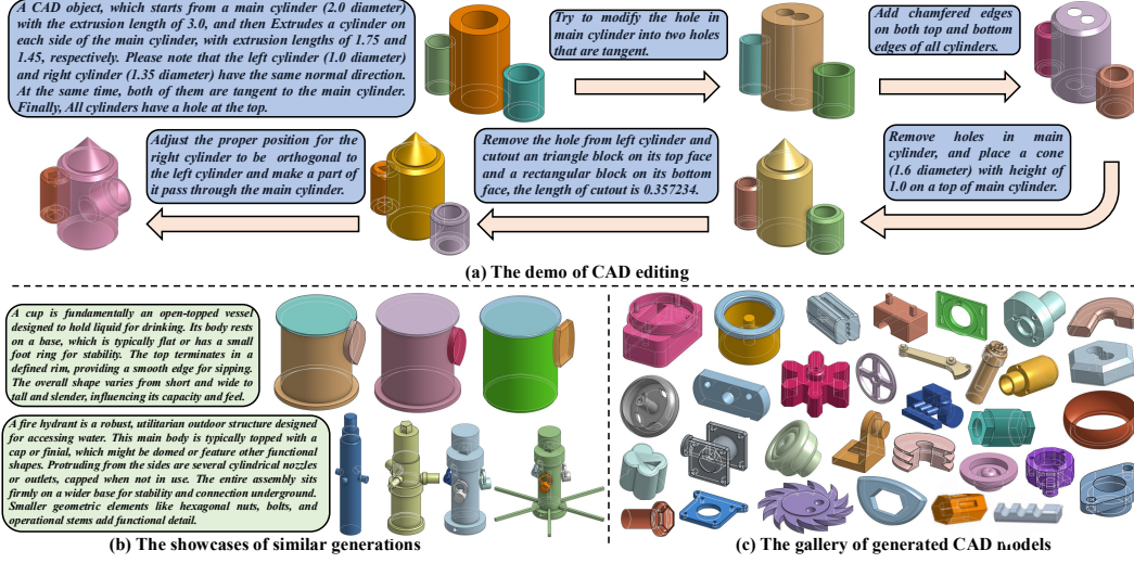
Figure 5: Various Showcases by Seek-CAD. Please enlarge to 180% to see the text clearly.
