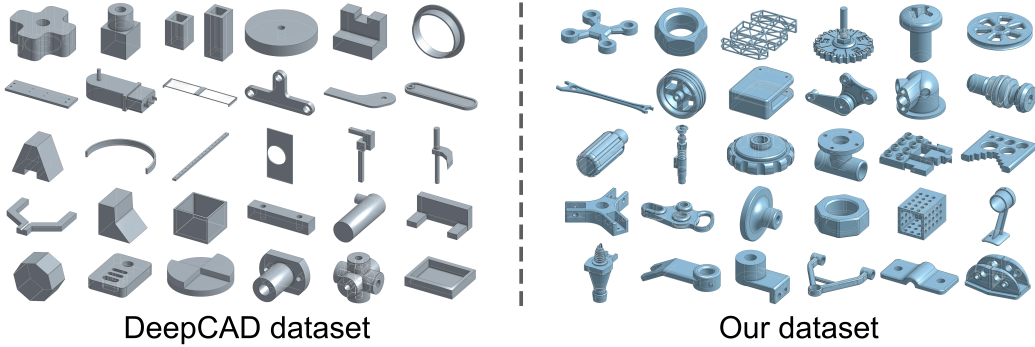
Figure 7: Qualitative comparison between our dataset and the DeepCAD [54] dataset. Compared to DeepCAD, our dataset captures more realistic and structurally complex industrial designs, supporting a broader range of modeling operations such as spline, revolve, chamfer, fillet, and shell. Our extended dataset also features richer geometric details and greater diversity in modeling strategies.
